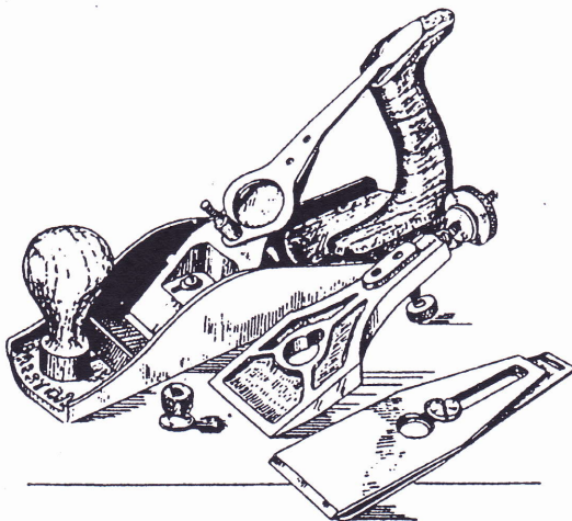
PRESTON'S PLANE TAKEN APART.
