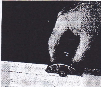
SURFORM MARKING GAUGE
